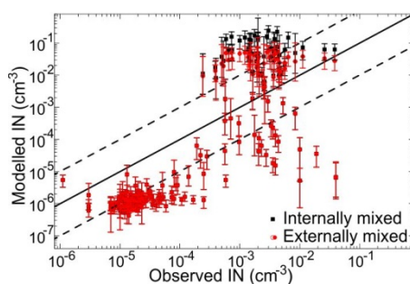
Supplementary Figure 8. Modelled versus observed K-feldspar IN concentrations, comparing different modelled mixing assumptions. Observations and annual mean modelled data ranges and sources are as in Figure 4f. In the internally mixed assumption, IN concentrations are calculated using Supplementary Equation 1 and the externally mixed assumption using Supplementary Equation 2. Vertical error bars represent the maximum and minimum modelled monthly mean values.
