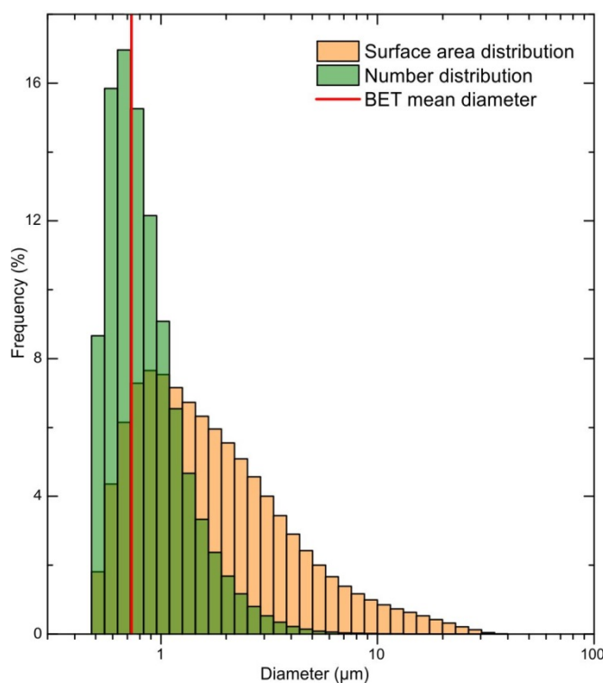
Supplementary Figure 5. Surface area and number distribution for the K-feldspar sample suspended in water. The mean surface area particle diameter from BET measurements (from Supplementary Table 3) is shown for comparison. The size distribution was measured using a Malvern Mastersizer 2000E laser diffraction instrument. The specific surface area calculated from this distribution is 0.89 \text{ m}^2 \text{ g}^{-1} , a factor of 3.5 smaller than that derived from the gas adsorption technique. Note that the laser diffraction technique is insensitive to the smallest particles in the distribution and this results in the distribution falling away too sharply at smaller sizes and an underestimate in specific surface area.
