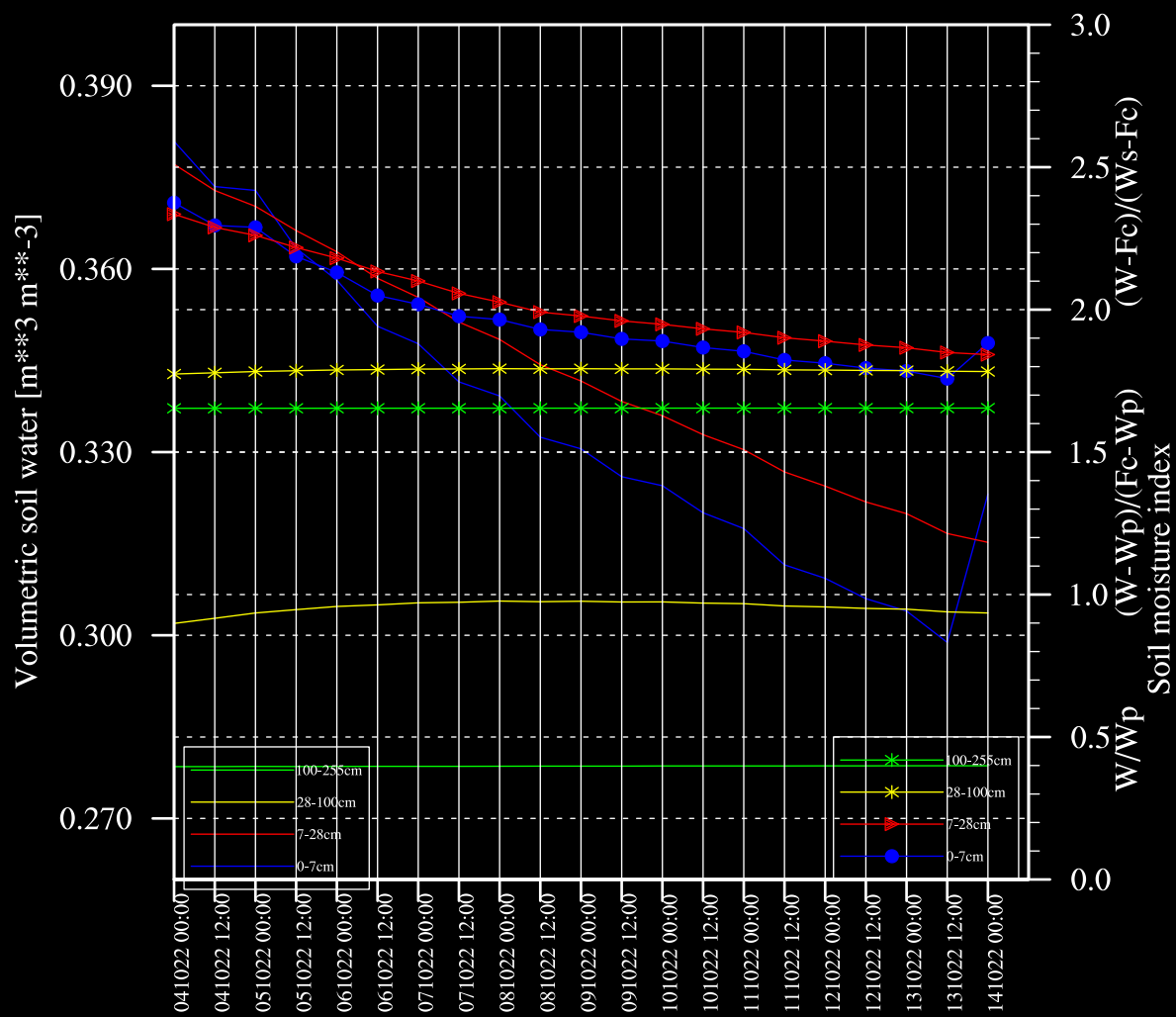
Aerodrom_Beograd, Volumetric soil water & SMI ECMWF 10/04/2022 (00:00)
