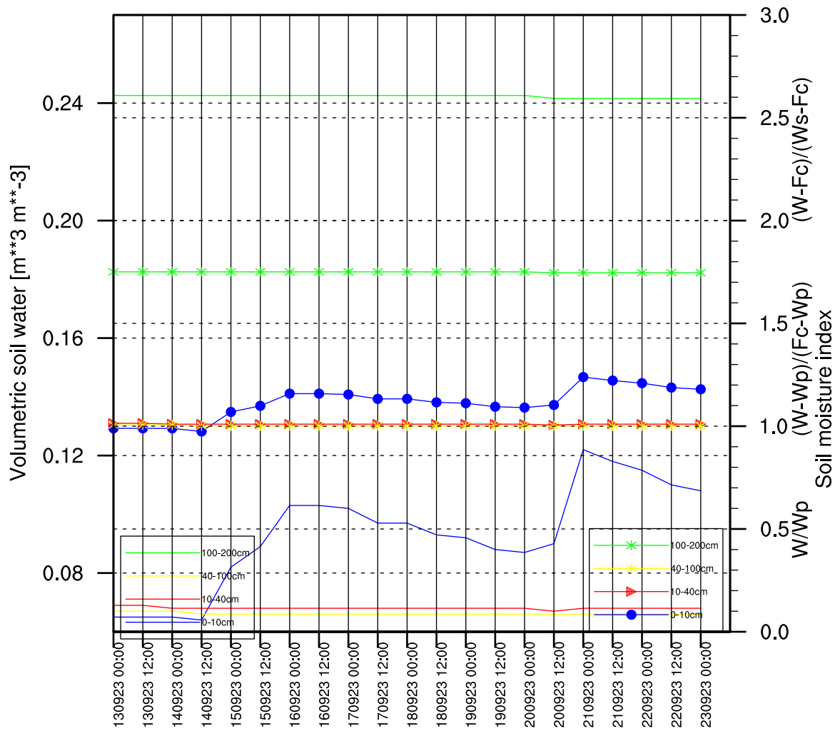
G_Aerodrom_Beograd, Volumetric soil water & SMI GFS 09/13/2023 (00:00)
