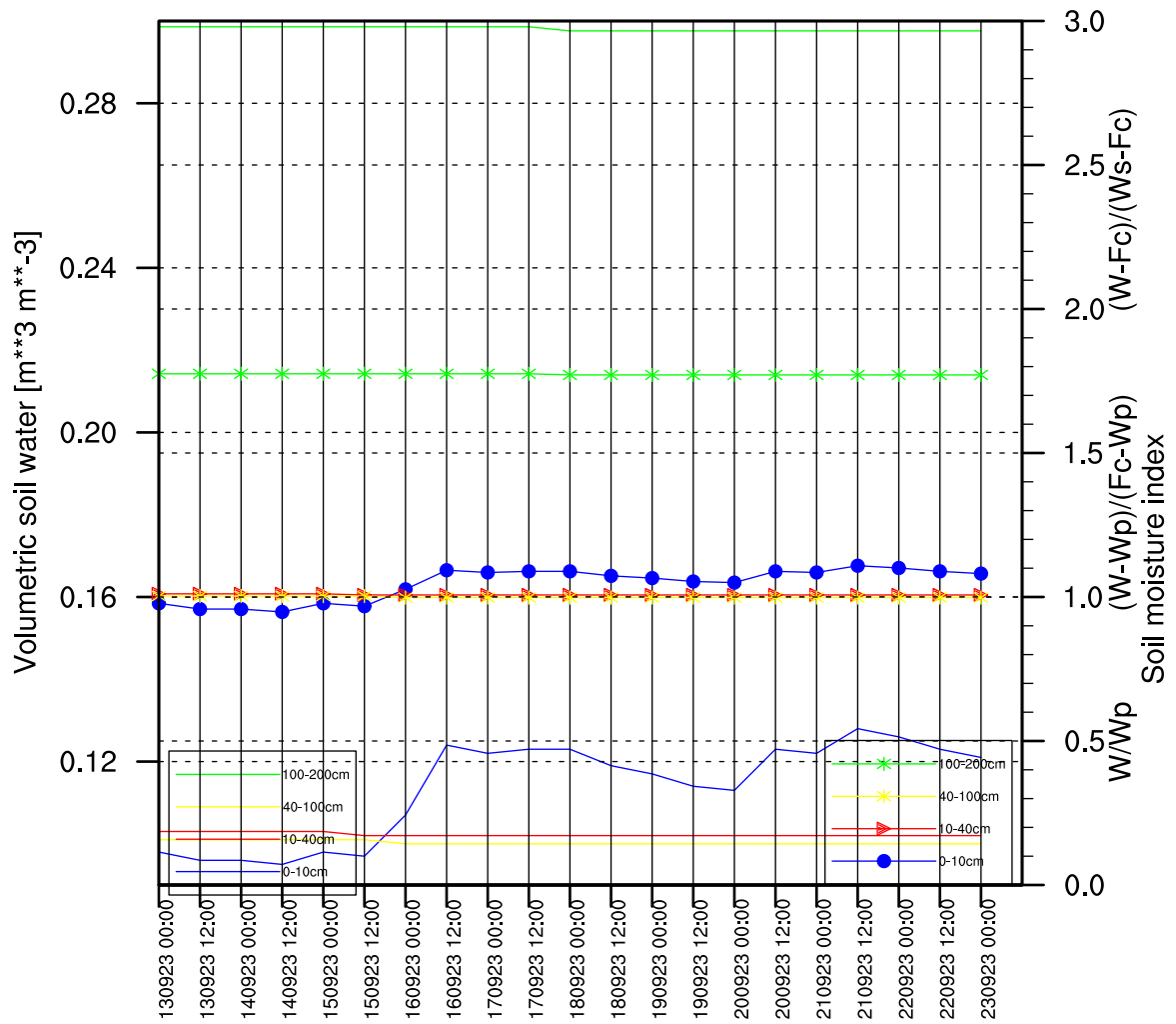
G_Aerodrom_Vr☆☆ac, Volumetric soil water & SMI GFS 09/13/2023 (00:00)
