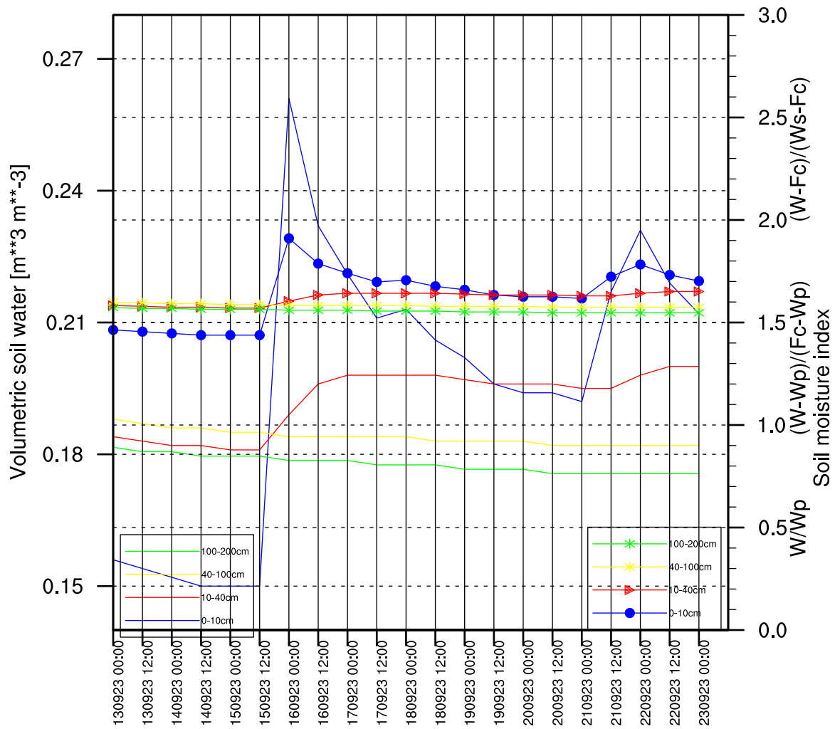
G_Kopaonik, Volumetric soil water & SMI GFS 09/13/2023 (00:00)
