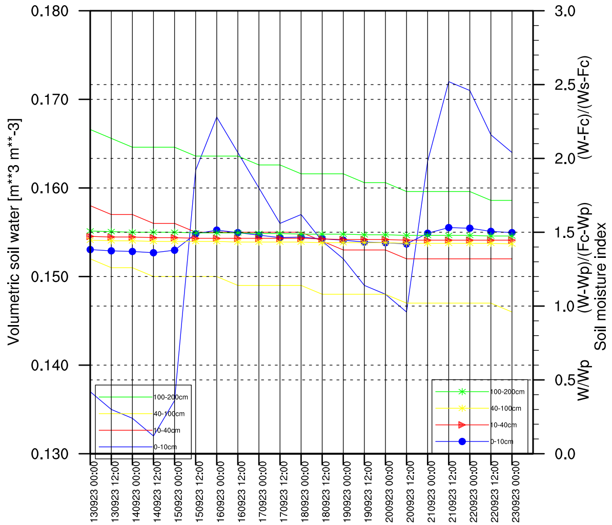
G_Kraljevo, Volumetric soil water & SMI GFS 09/13/2023 (00:00)
