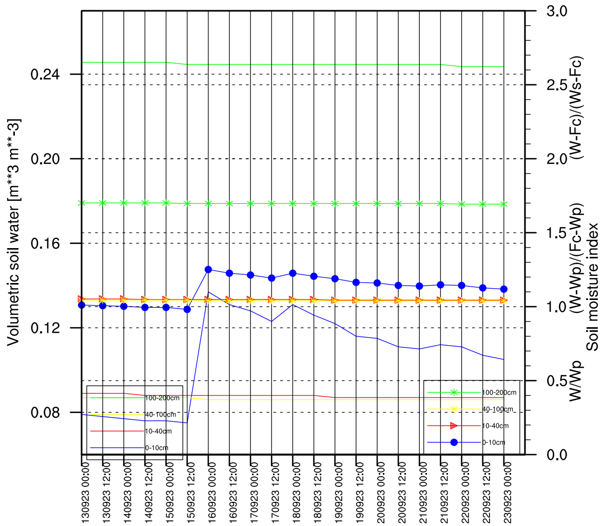
G_Kur☆☆umlija, Volumetric soil water & SMI GFS 09/13/2023 (00:00)
