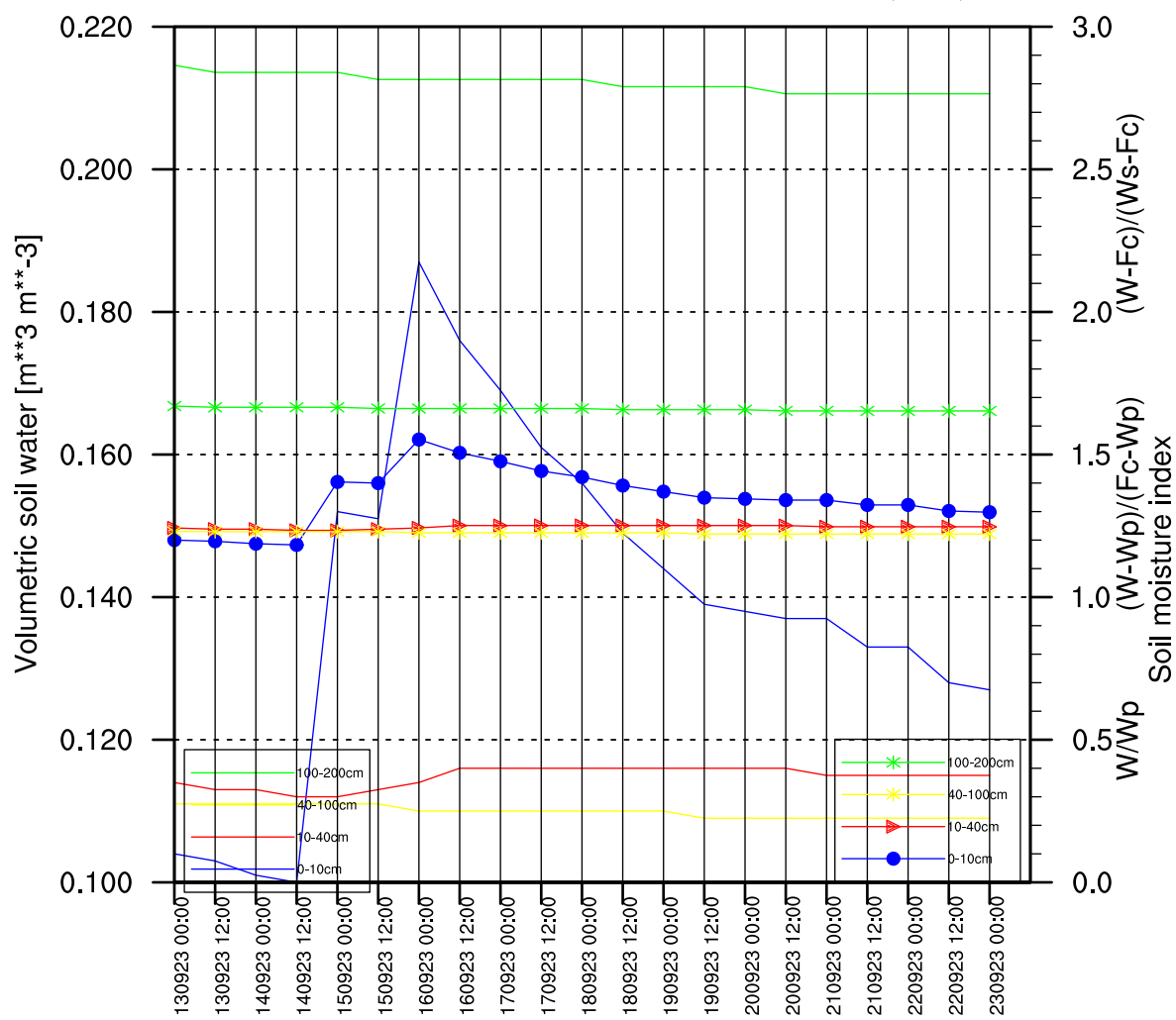
G_Loznica, Volumetric soil water & SMI GFS 09/13/2023 (00:00)
