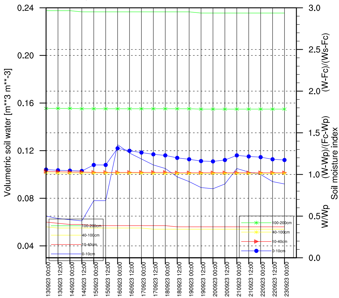
G_Valjevo, Volumetric soil water & SMI GFS 09/13/2023 (00:00)
