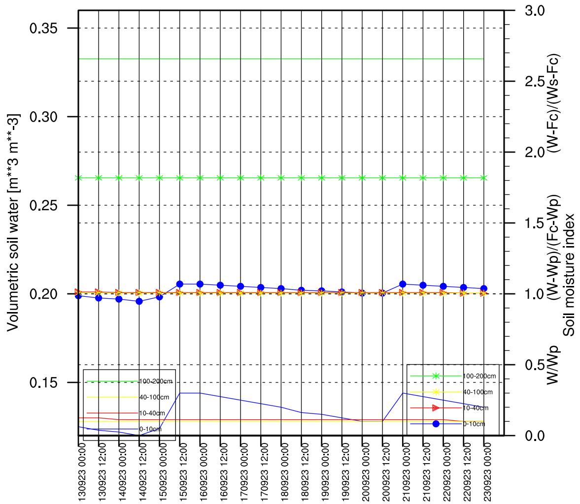
G_Zaje☆ar, Volumetric soil water & SMI GFS 09/13/2023 (00:00)
