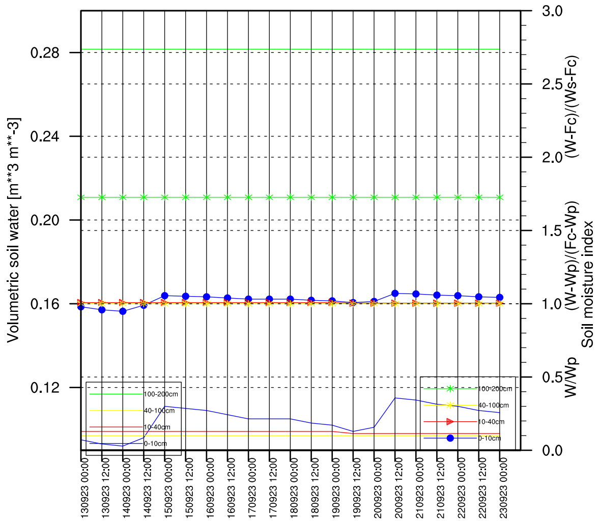
G_Zrenjanin, Volumetric soil water & SMI GFS 09/13/2023 (00:00)
