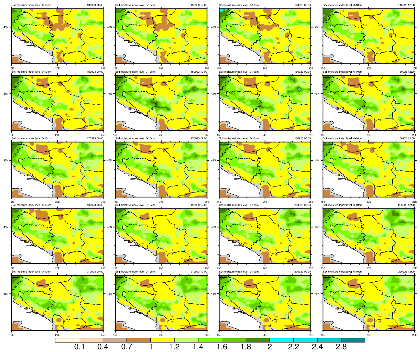
Soil moisture index GFS level 0-10cm 09/13/2023 (00:00)
