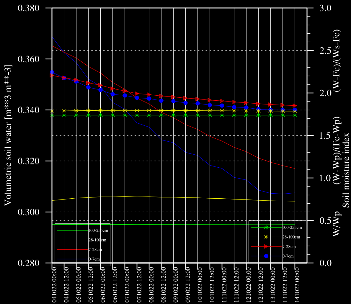
Kopaonik, Volumetric soil water & SMI ECMWF 10/04/2022 (00:00)
