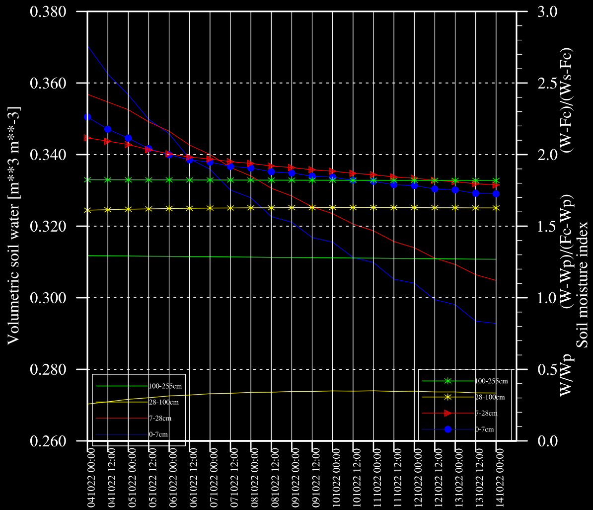
Leskovac, Volumetric soil water & SMI ECMWF 10/04/2022 (00:00)
