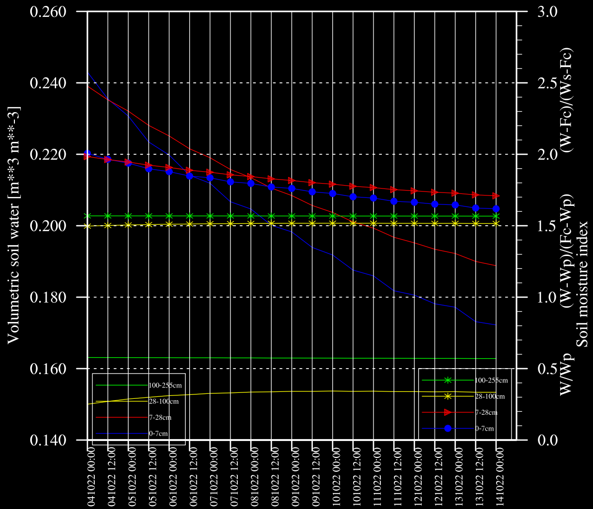
Pali☆☆, Volumetric soil water & SMI ECMWF 10/04/2022 (00:00)
