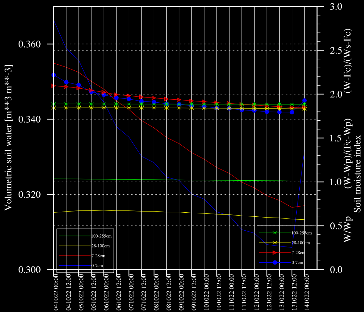
Porto Alegre, Volumetric soil water & SMI ECMWF 10/04/2022 (00:00)
