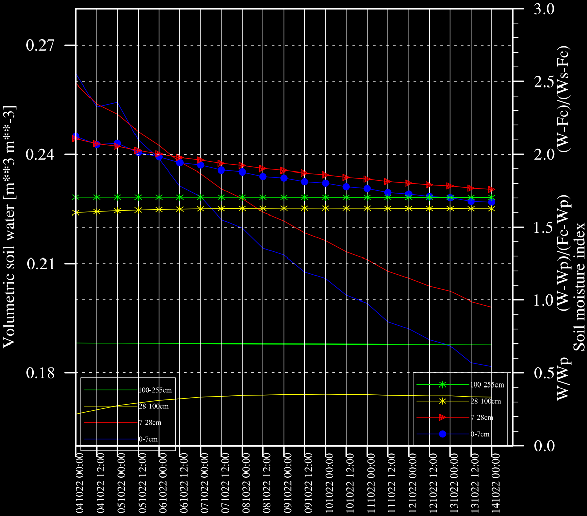
Rimski_☆an☆☆vi, Volumetric soil water & SMI ECMWF 10/04/2022 (00:00)
