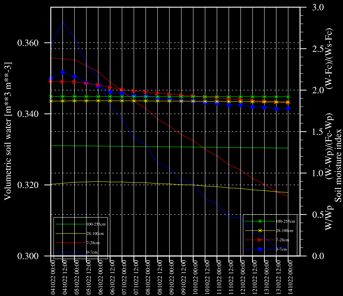
Sjenica, Volumetric soil water & SMI ECMWF 10/04/2022 (00:00)
