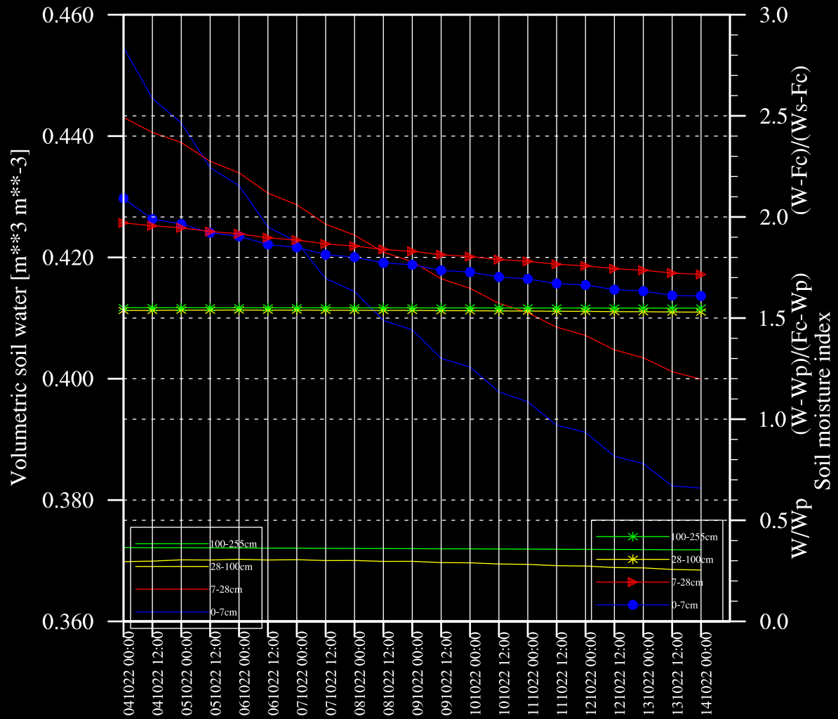
Zaječar, Volumetric soil water & SMI ECMWF 10/04/2022 (00:00)
