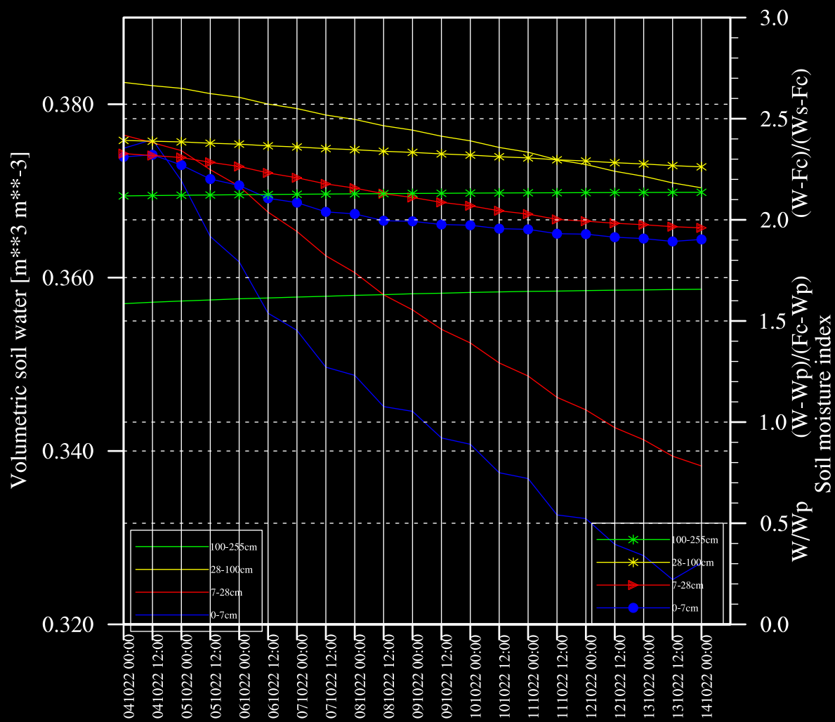
Zlatibor, Volumetric soil water & SMI ECMWF 10/04/2022 (00:00)
