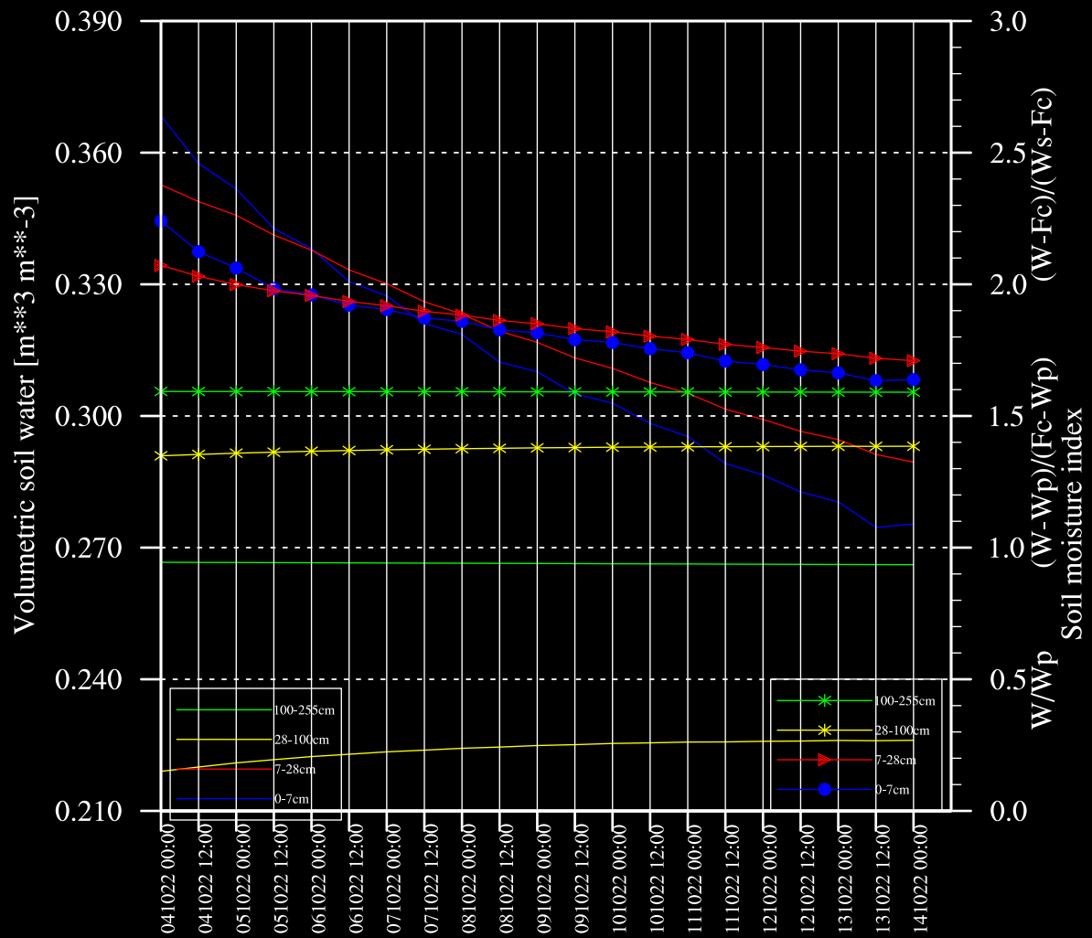
Zrenjanin, Volumetric soil water & SMI ECMWF 10/04/2022 (00:00)
