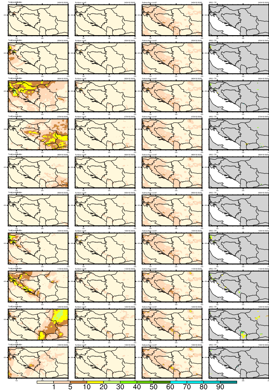
TP, SRO, SSRO [mm] & SRO/TP, ECMWF, start 04/03/2018 (00:00)
