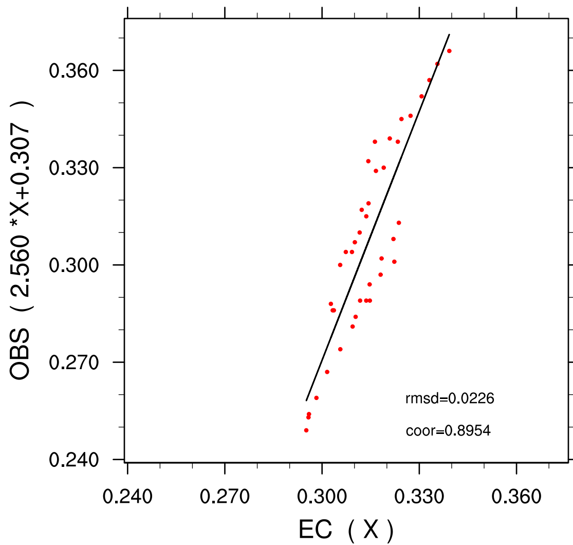
Beograd_Vracar EC-OBS APR dec=3
