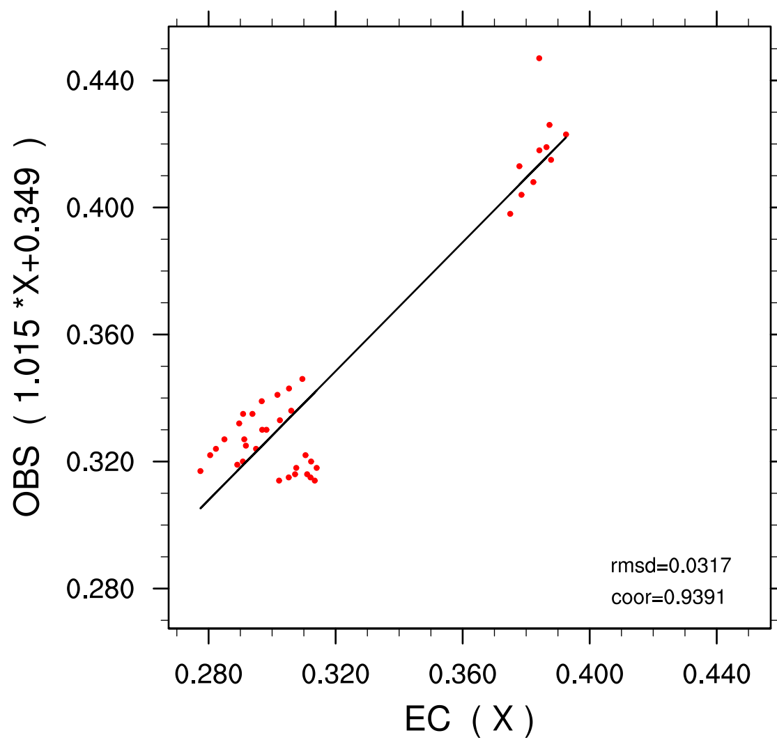
Leskovac EC-OBS MAY dec=1
