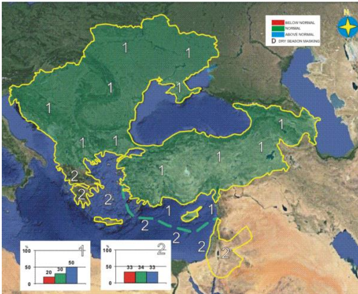
Fig 2. SEECOF-30 precipitation outlook for 2023-2024.
