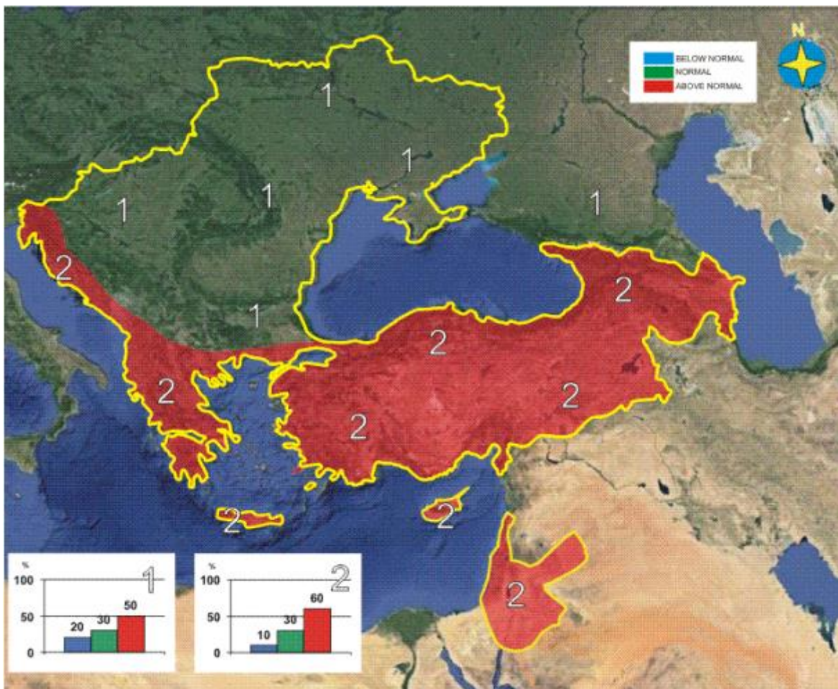
Fig 1. SEECOF-30 temperature outlook for 2023-2024.
