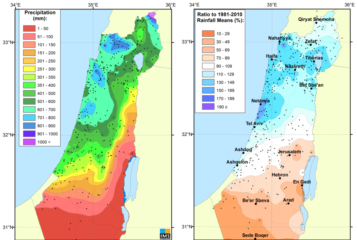
Fig 4. (a) DJF 2023/24 accumulated precipitation (mm). (b) Percent of normal (1981-2010).
