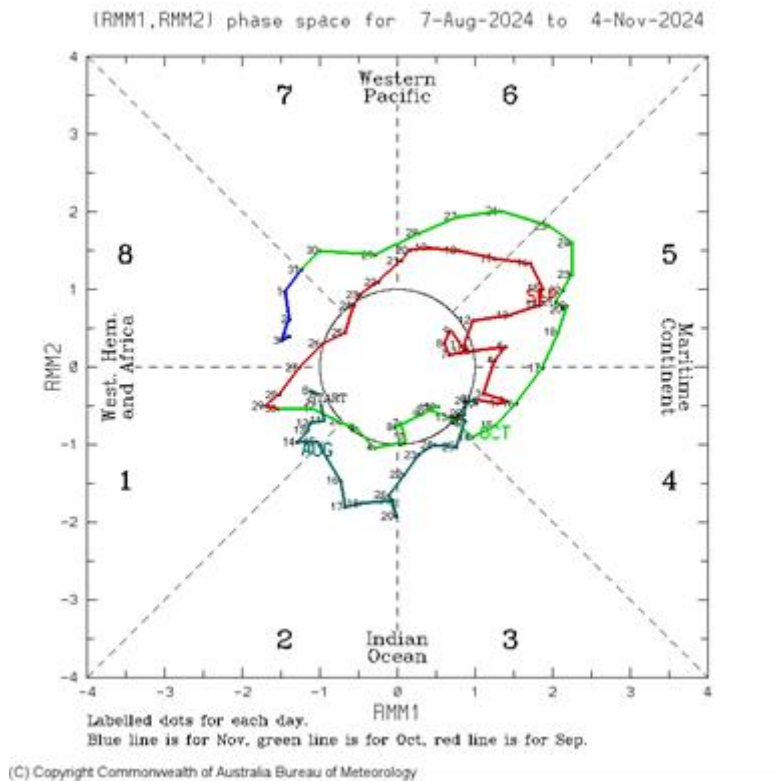
Fig. 2.8: MJO phase diagram August-November 2024. Source: http://www.bom.gov.au/climate/mjo/
