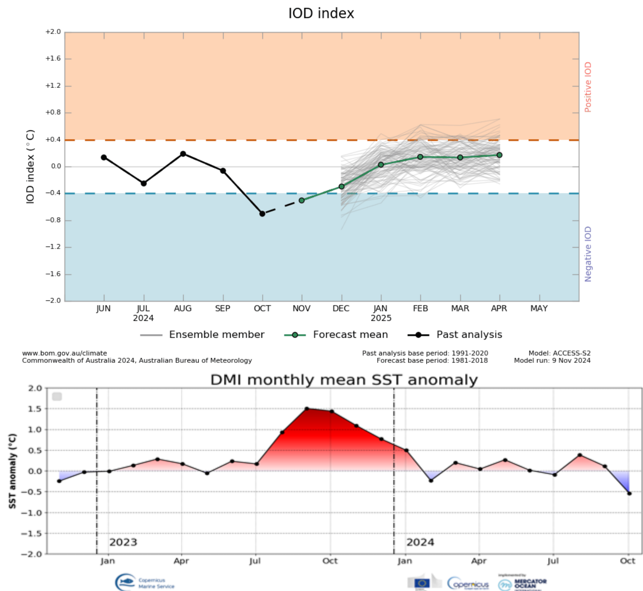
Figure 1.5 Observed and expected evolution of Indian Ocean Dipole. Source: upper map: BOM, http://www.bom.gov.au/climate/ensio/index.shtml#tabs=Indian-Ocean ), lower map: Météo France, Mercator Ocean data
