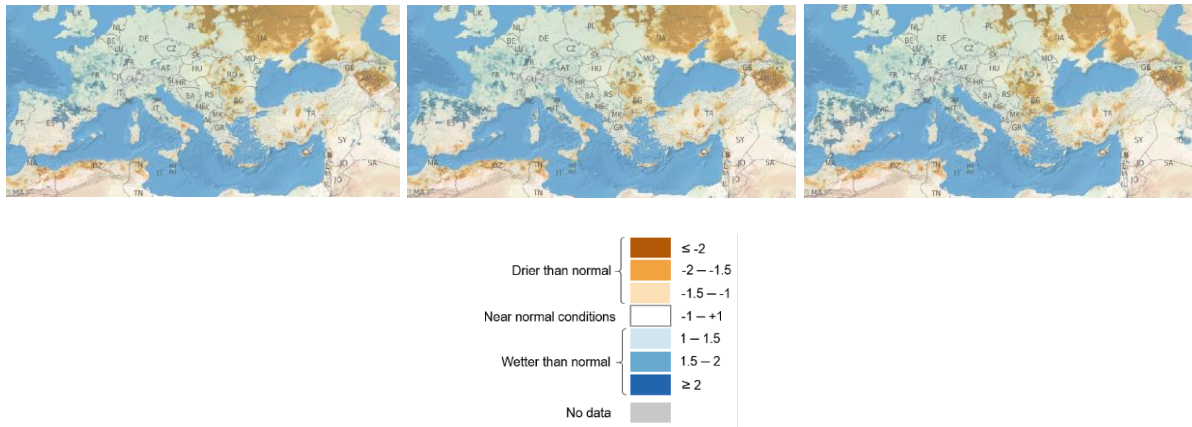
Figure 6.1: 10-day anomalies of soil moisture index (SMI) in October 2024, reference period: 1995-2023. Source: European Drought Observatory (EDO), https://edo.jrc.ec.europa.eu/edov2/php/index.php?id=1111
