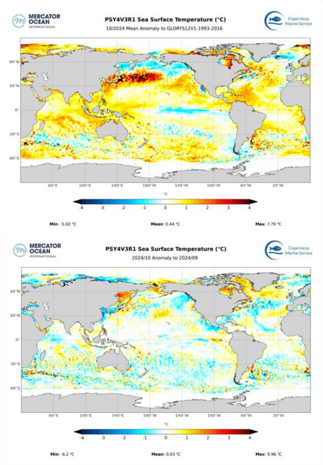
Figure 1.1: Upper map: sea surface temperature anomalies for October 2024. Lower map: anomaly differences October minus September 2024 (anomaly trend). Source: Météo France, Mercator Ocean data.
